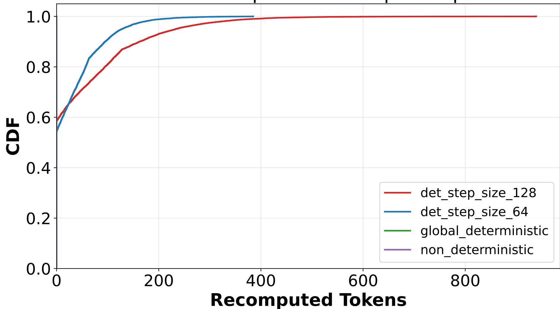
CDF of Recomputed Tokens per Request
