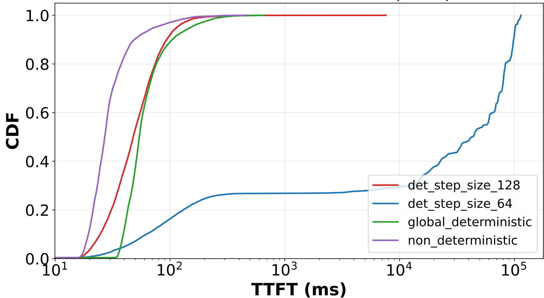
CDF of Time To First Token (TTFT)
