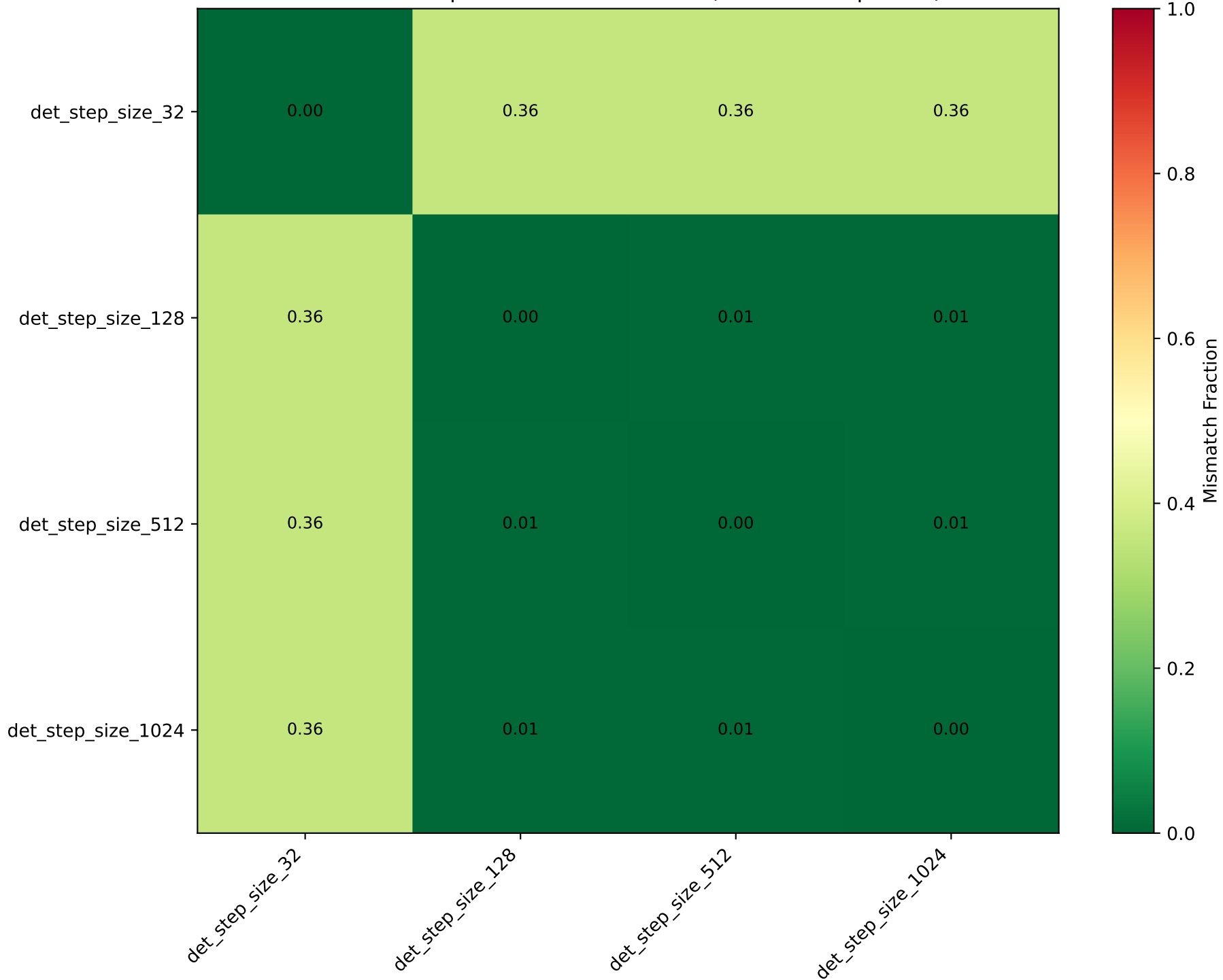
Pairwise Output Mismatch Fractions (Different Step Sizes)
