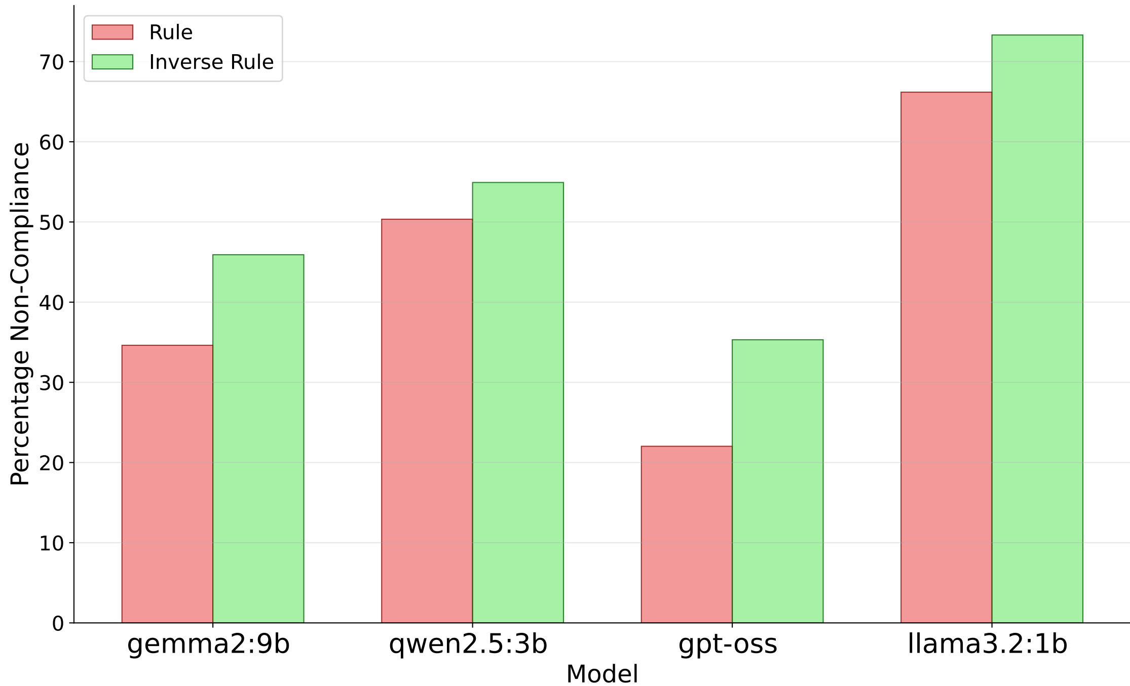
Rule vs Inverse Rule Non-Compliance
