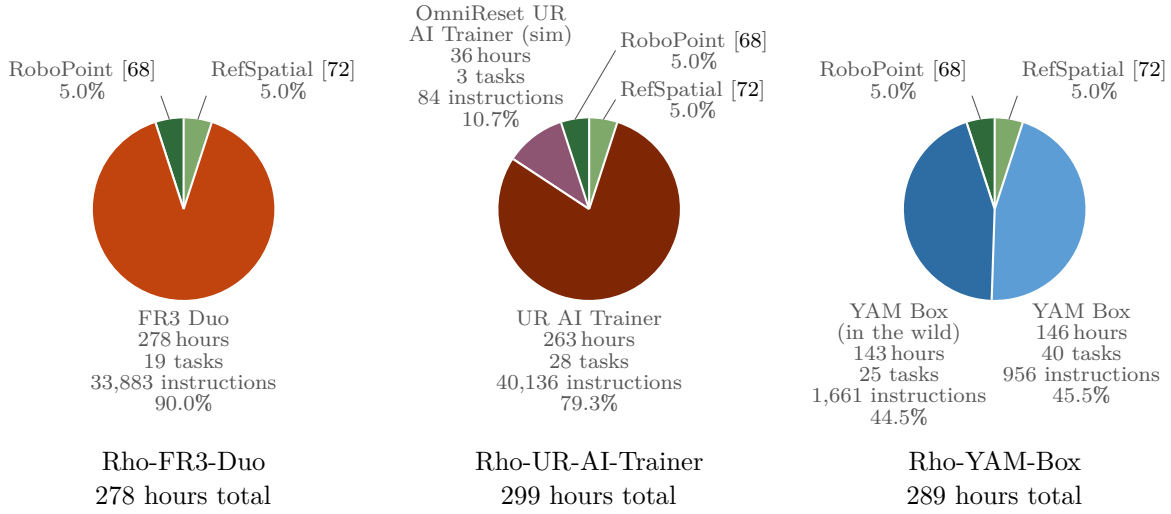
Figure 4 Midtraining mixtures of the embodiment-specific Rho variants. The count of distinct language instructions includes the number of both task and subtask descriptions.
