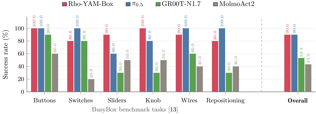
Figure 8 YAM Box results. Rho-YAM-Box outperforms all baselines except \pi_{0.5} , which had thousands of hours of training data from robots similar to YAM Box, and is essentially midtrained on this embodiment.
