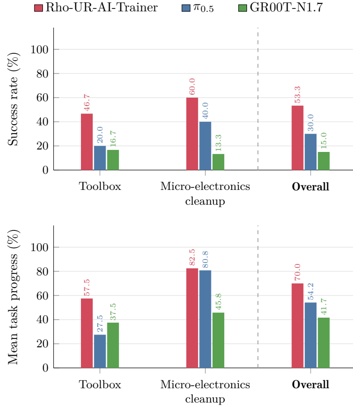
Figure 9 UR AI Trainer results. Rho-UR-AI-Trainer dominates in terms of success rate and is matched by \pi_{0.5} on the Micro-electronics Cleanup task. The reason is different failure modes of Rho and \pi_{0.5} . The former sometimes fails to pick up one of the small electronics chips, failing early in these cases, but precisely places picked-up electronics into the tray. \pi_{0.5} , in contrast, tends to fail at precision placement, at the last stage of the task.
