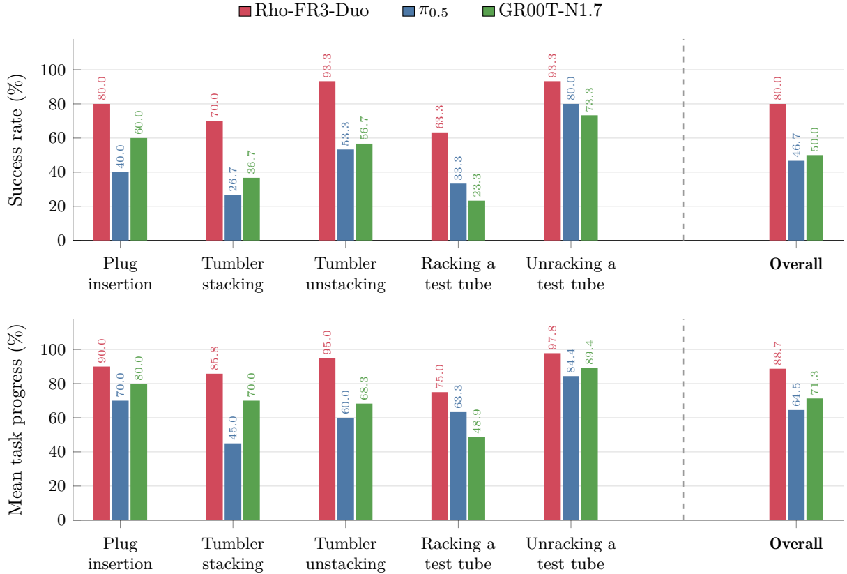
Figure 10 FR3 Duo task-adaptation results. Each model is adapted independently on each task dataset and evaluated over 30 distinct, matched initial configurations per variant. We report binary success rate and mean task progress; Overall is the unweighted mean across the five task variants.
