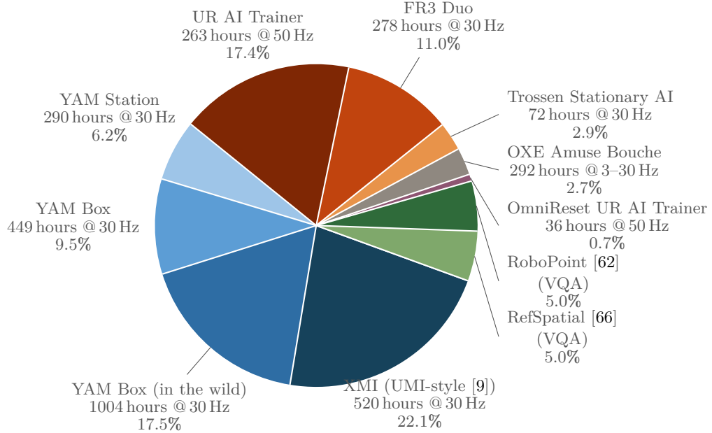
Figure 3 Rho-Tomyum mixture. It consists of 90% robot and UMI-style data and 10% vision-language data. All the robot/UMI-style data is bimanual, with the exception of a small subset of Open X-Embodiment Magic Soup [3] we call OXE Amuse Bouche . The robot data includes trajectories from policies controlling a UR AI Trainer simulated in NVIDIA Isaac Sim, trained using RL and the OmniReset framework [59].
