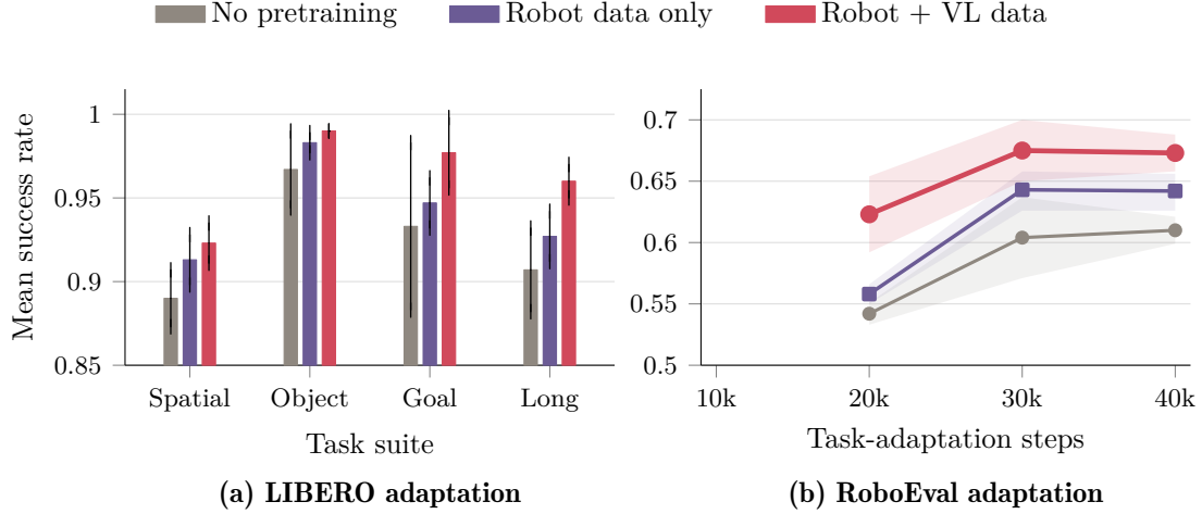
Figure 4 Pretraining on 15% of the dataset mixture improves downstream adaptation. Left: LIBERO suite success after 20k task-adaptation steps. Right: RoboEval success throughout adaptation. The robot+VL condition combines robot trajectories with physical-grounding examples, the robot-data-only condition removes the physical-grounding batches, and the no-pretraining condition begins task adaptation from the grounded backbone with a randomly initialized action expert. Values are means and standard deviations over three evaluations, except the robot+VL RoboEval result at 40k adaptation steps, which pools six passes from two independent evaluations.
