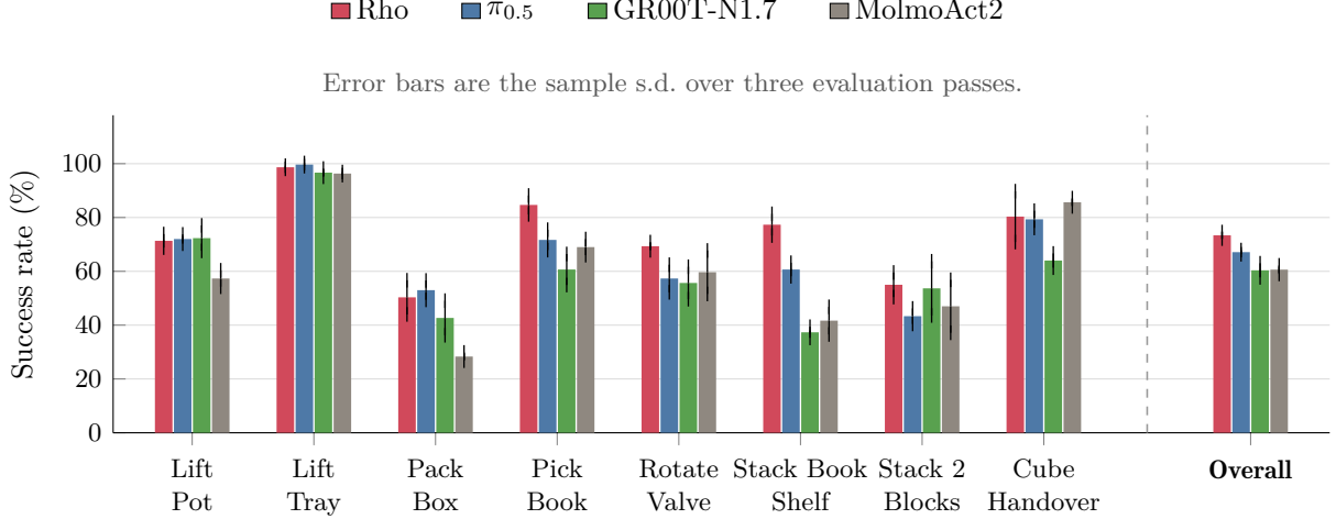
Figure 7 RoboEval results caption
