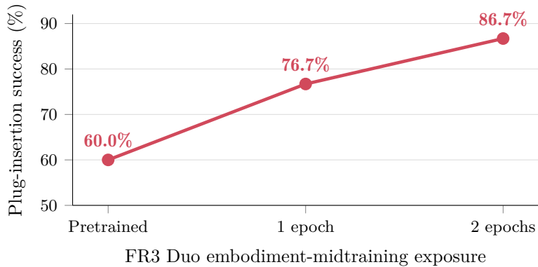
Figure 6 FR3 Duo horizontal midtraining improves subsequent vertical adaptation to bimanual plug insertion. Every condition uses the same 50k-step task-adaptation budget; success reported over 30 trials.
