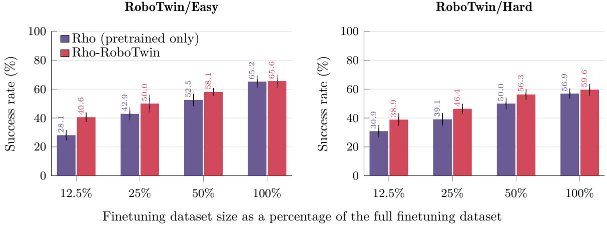
Figure 5 Embodiment midtraining on RoboTwin transfers to held-out tasks across downstream-data budgets. Each checkpoint is adapted for 40k steps and evaluated on the matched five-task protocol with 50 episodes per task. Bars are means over completed seeds (four for Easy, three for Hard) and error bars are sample standard deviations. The benefit of midtraining is largest in the low-data regime and shrinks as the adaptation set grows.
