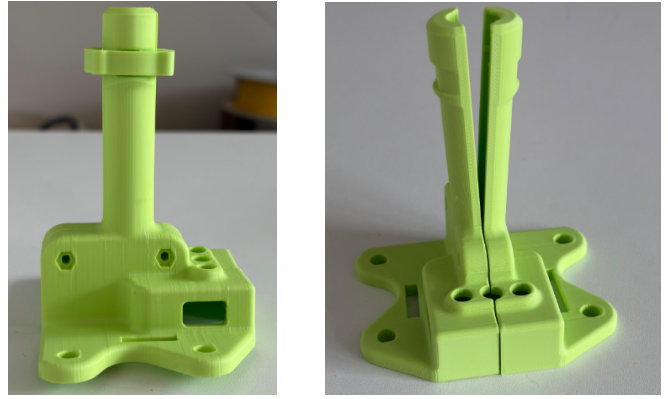
Fig. 5: Final Design with clip on/off
