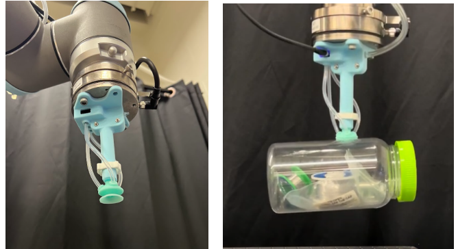
(a) Final prototype mounted on robot arm (b) Final prototype grasping transparent, oddly shaped object
