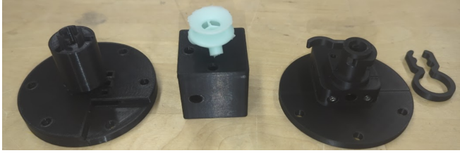
Fig. 3: Three concepts first prototype (Twist-fit, Press-fit, Clip)
