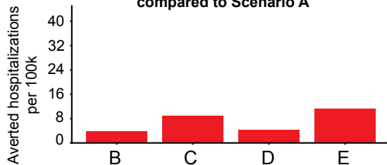
C Scenario effect on winter wave size compared to Scenario A
