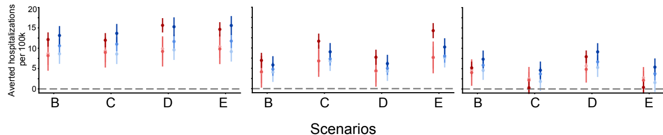
Model 4
