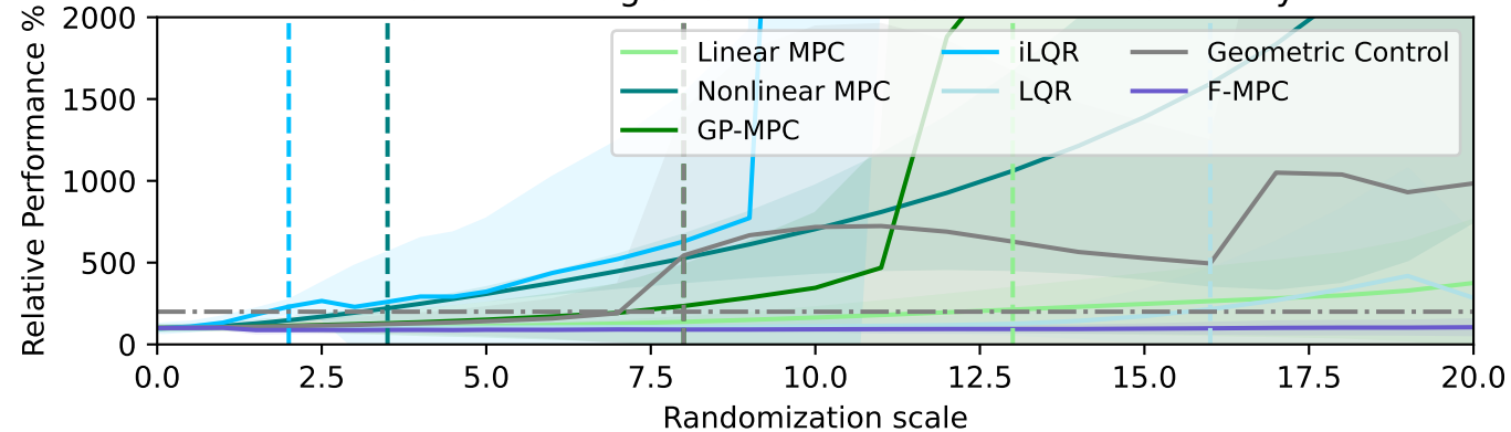
Performance Degradation with Parametric Uncertainty
