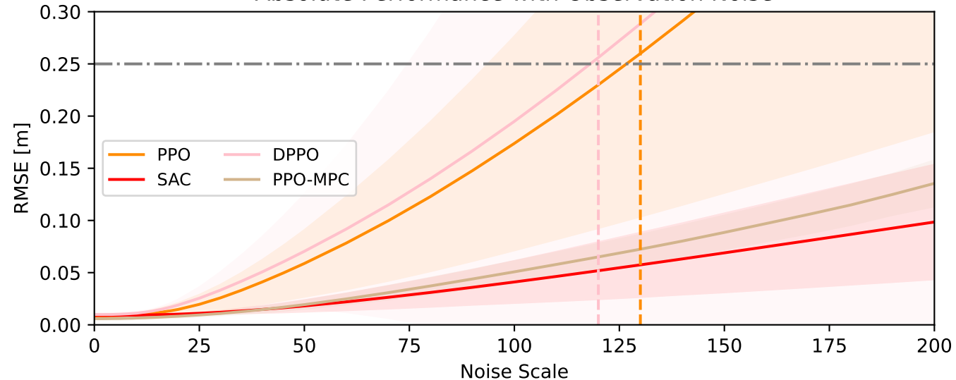
Absolute Performance with Observation Noise
