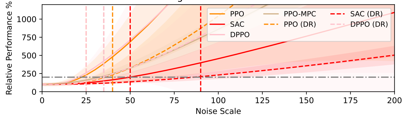
Performance Degradation with Observation Noise
