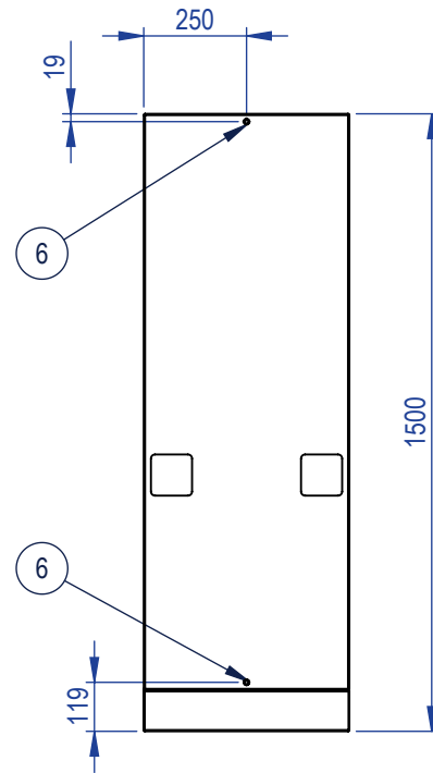
PLAN VIEW
