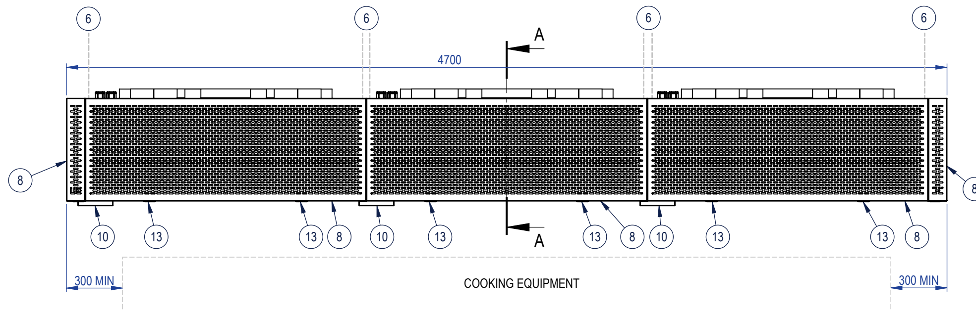
FRONT VIEW
