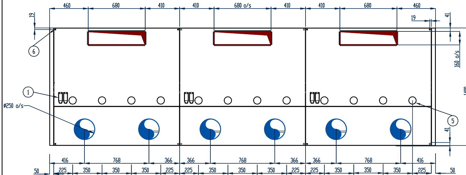
PLAN VIEW
