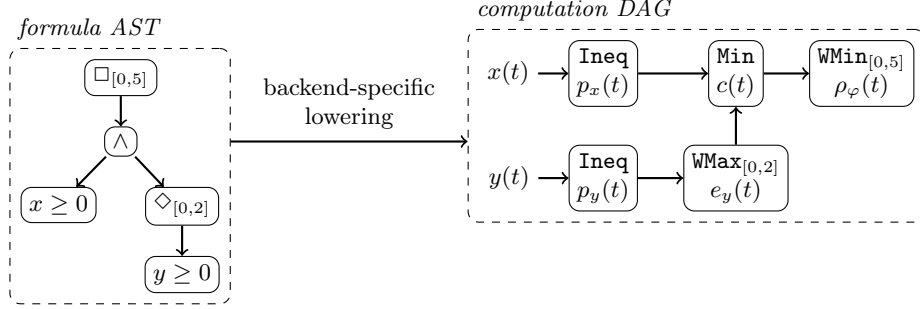
Fig. 2. Lowering of \varphi \equiv \Box_{[0,5]}((x \geq 0) \wedge \Diamond_{[0,2]}(y \geq 0)) from the formula AST (left) to a computation DAG (right). Nodes are typed primitive operations ( Min is point-wise; WMax / WMin aggregate over the annotated window); edges carry the intermediate robustness signals, which remain inspectable in the evaluation result.
