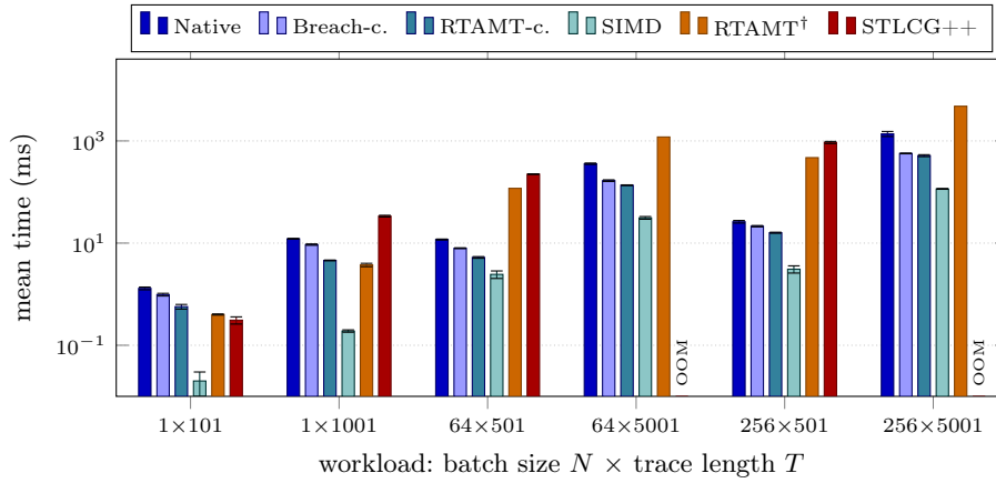
Fig. 4. Mean evaluation time on representative workloads, plotted on a log scale. All bars use the same formula \Box_{[0,5]}((x > 0) \wedge \Diamond_{[0,2]}(y > 0)) ; error bars show one standard deviation. RTAMT † batch times are N \times the measured per-trace time; missing STLGG++ bars exceed memory (OOM).
