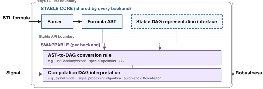
Fig. 1. Architecture of tidySTL: a stable core shared by every backend and a swappable backend layer (lowering and node interpretation) that isolates the implicit semantic choices.
