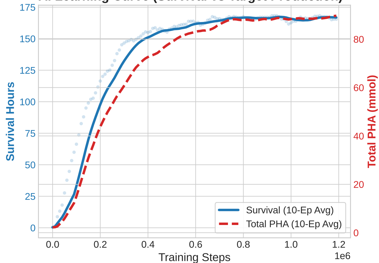
A. Learning Curve (Survival vs Target Production)
