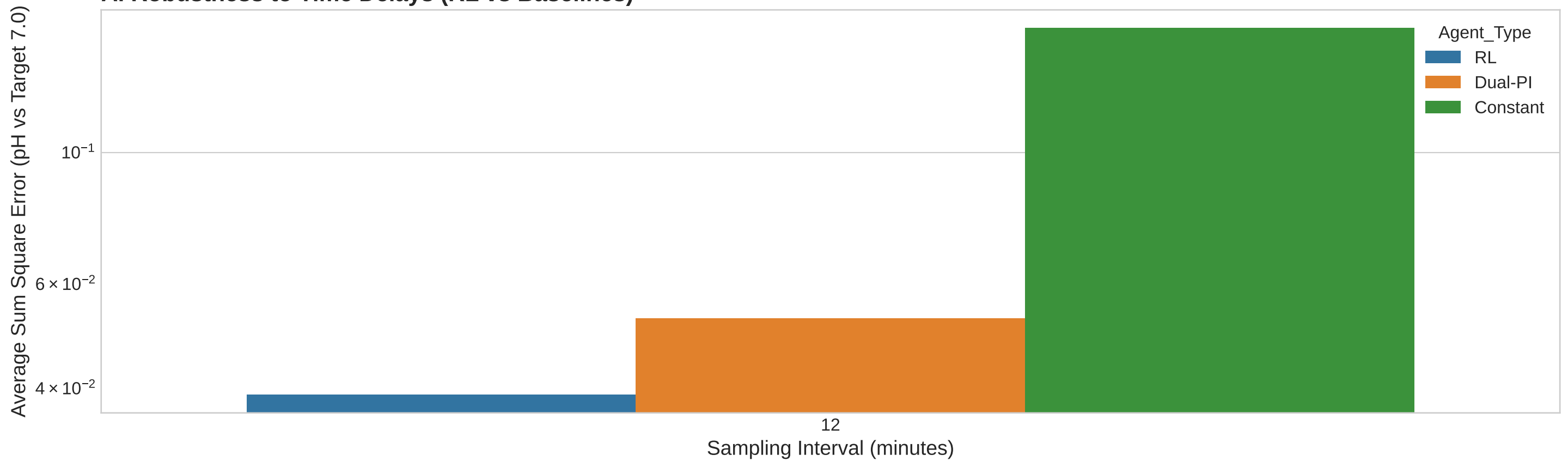
A. Robustness to Time Delays (RL vs Baselines)
