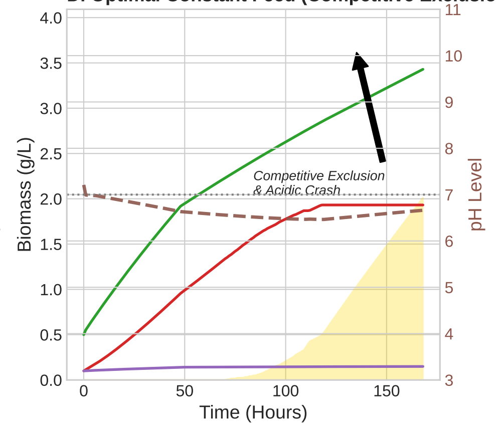
D. Optimal Constant Feed (Competitive Exclusion)
