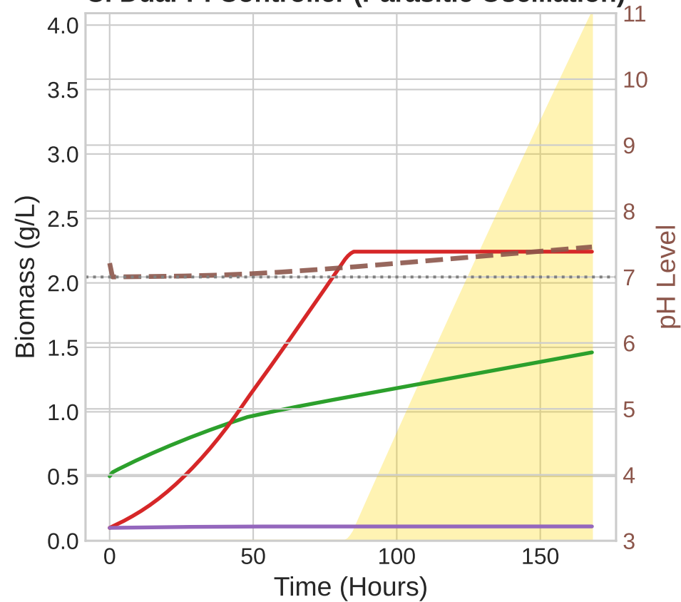
C. Dual-PI Controller (Parasitic Oscillation)
