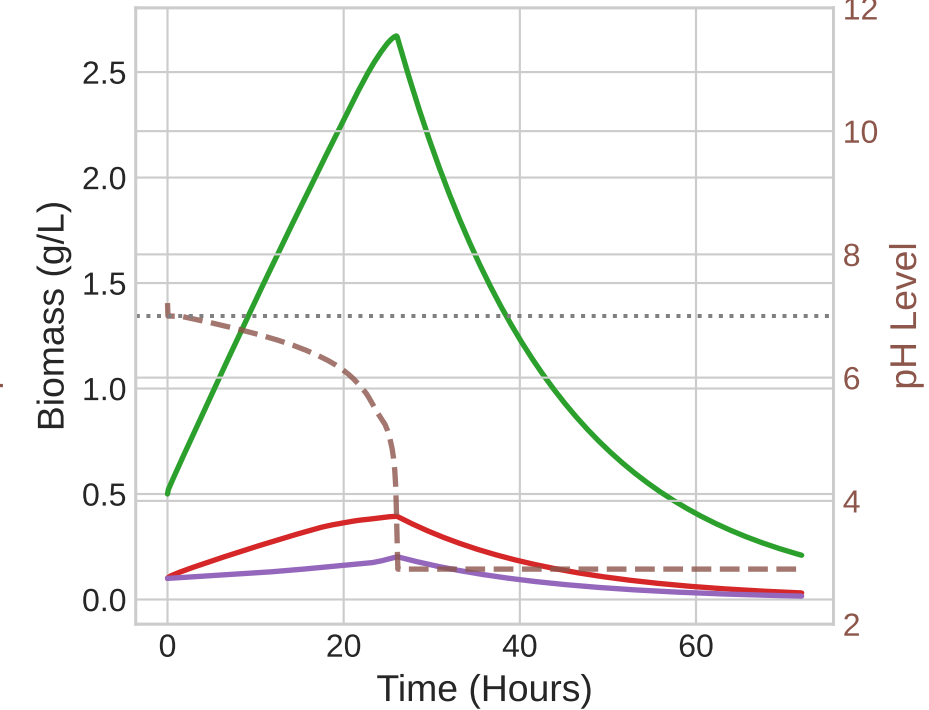
E. PI Control (12 min interval)
