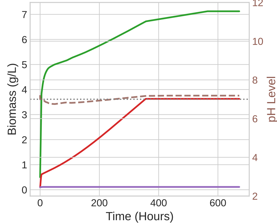
D. RL Control (12 min interval)
