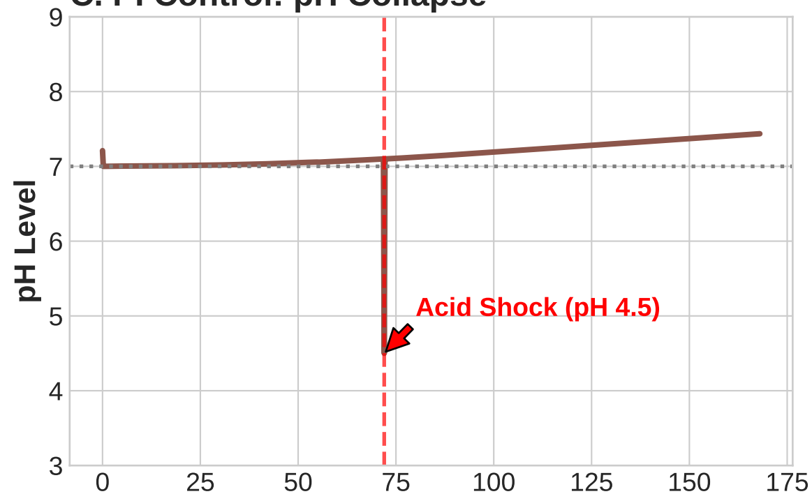
C. PI Control: pH Collapse
