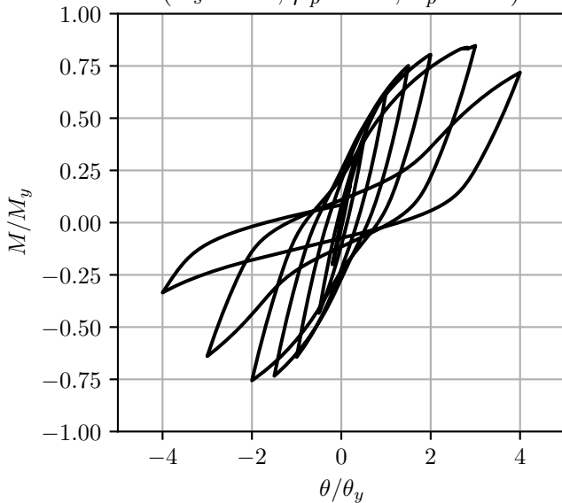
(c) Proposed BW ( R_s = 0.9, \mu_p = 3.0, \sigma_p = 1.0 )
