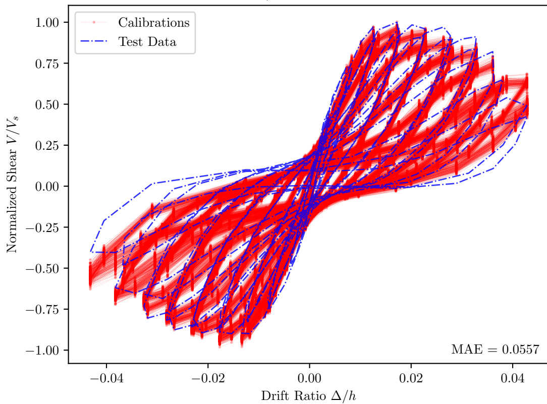
Ohue et al. 1985, 2D16RS — PEER Id = 033
