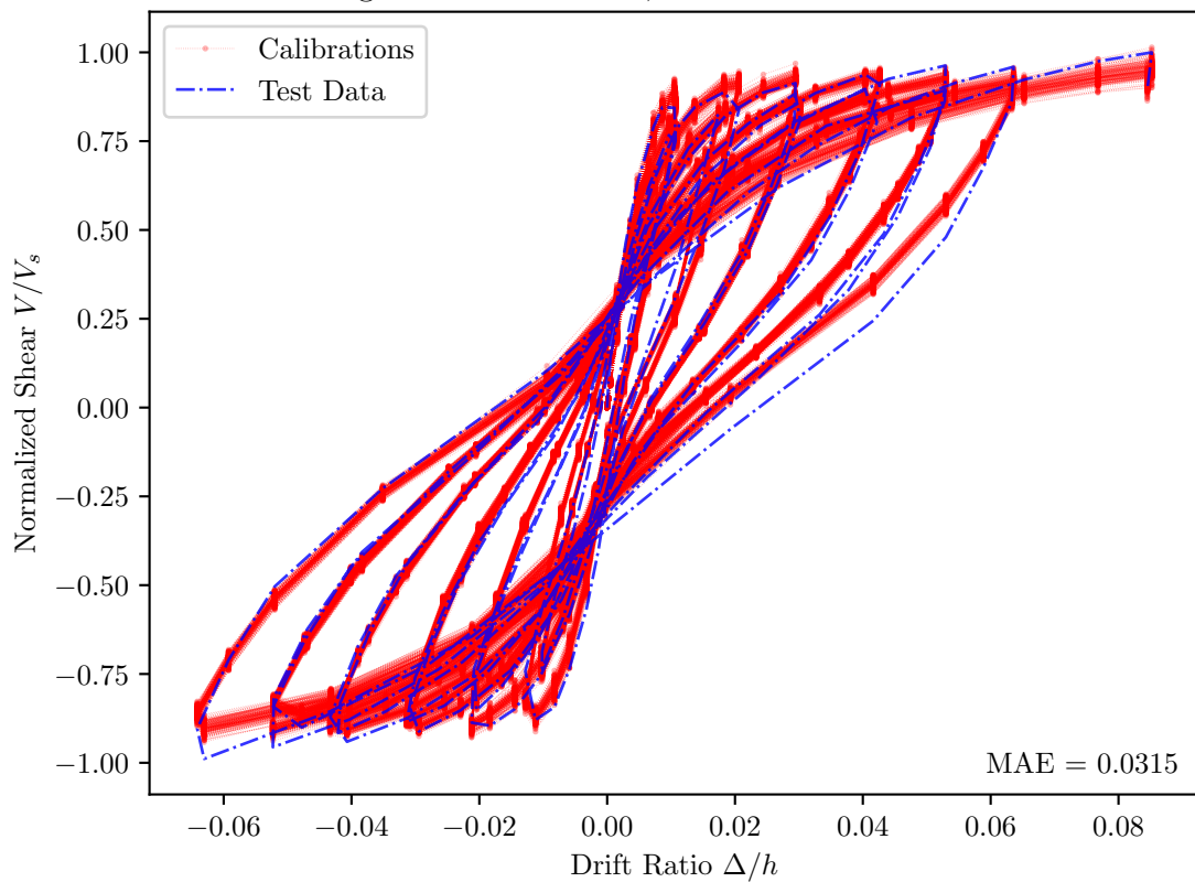
Muguruma et al. 1989, BH-1 — PEER Id = 061
