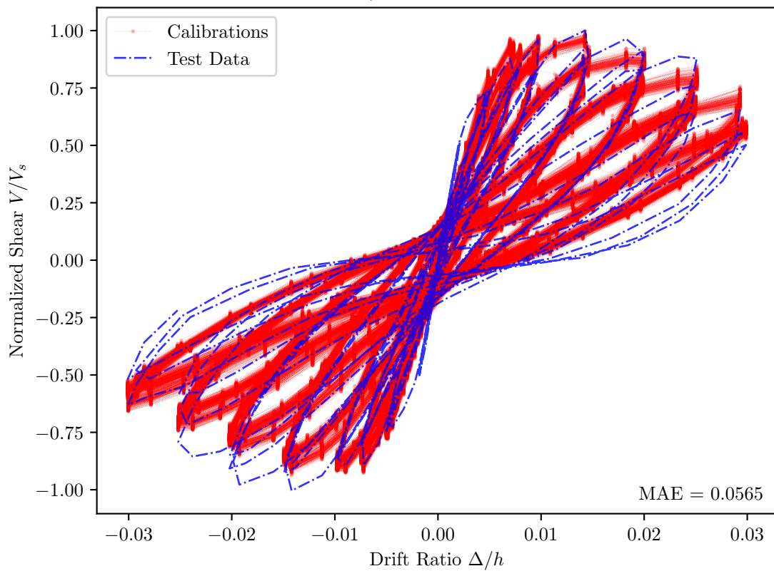
Ono et al. 1989, CA025C — PEER Id = 064
