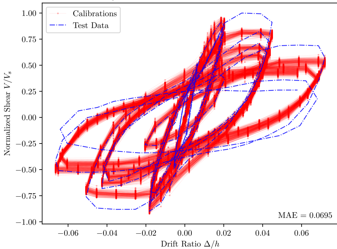
Saatcioglu and Ozcebe 1989, U3 — PEER Id = 105
