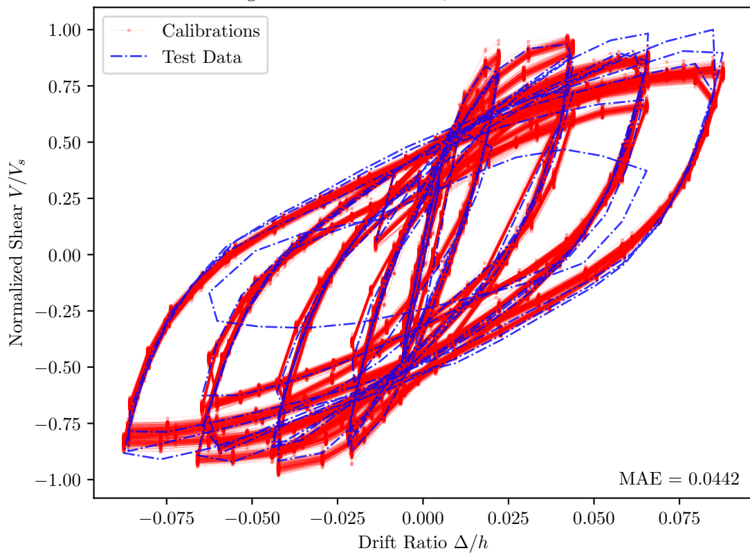
Saatcioglu and Ozcebe 1989, U7 — PEER Id = 108
