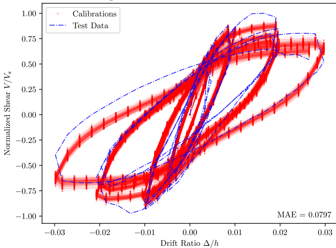
Saatcioglu and Grira 1999, BG-1 — PEER Id = 165
