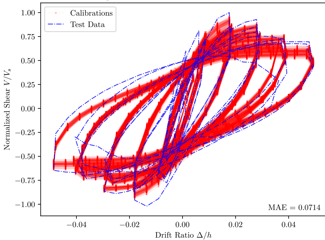
Saatcioglu and Grira 1999, BG-4 — PEER Id = 168
