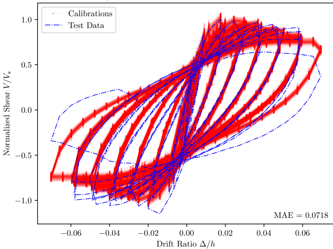
Saatcioglu and Grira 1999, BG-5 — PEER Id = 169
