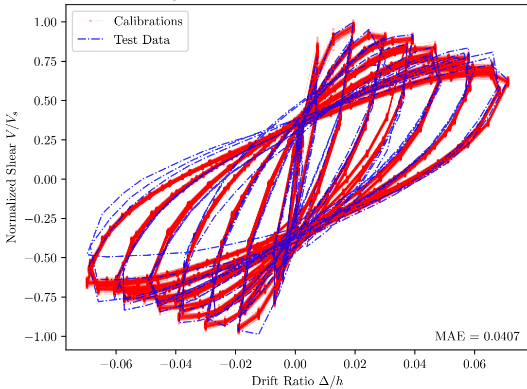
Saatcioglu and Grira 1999, BG-9 — PEER Id = 173
