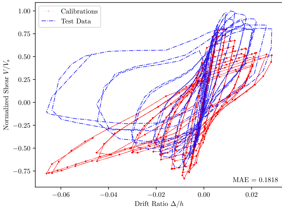
Thomsen and Wallace 1994, B3 — PEER Id = 205
