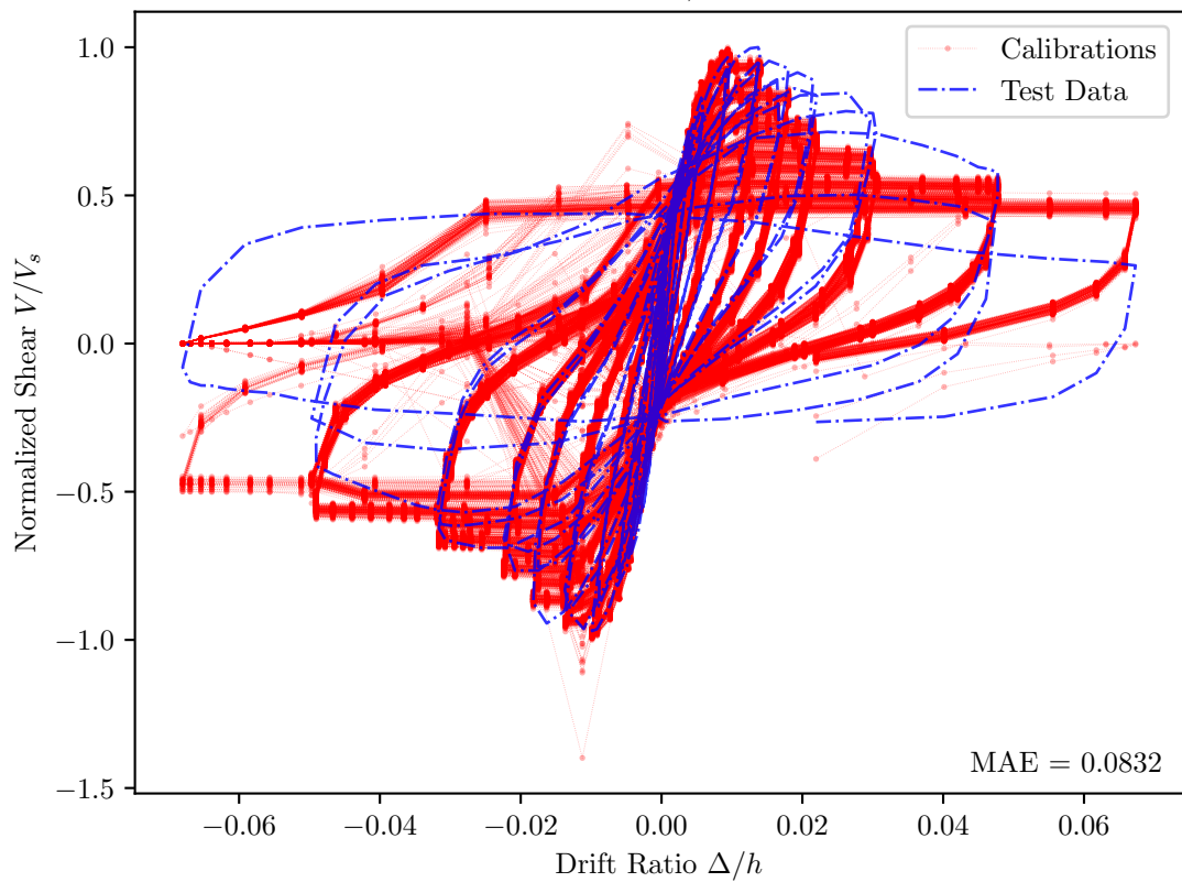
Thomsen and Wallace 1994, C3 — PEER Id = 208
