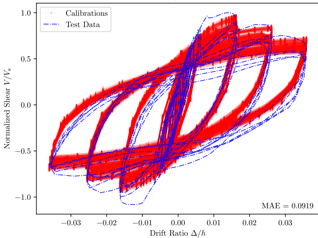
Petrovski and Ristic 1984, M1E1 — PEER Id = 299
