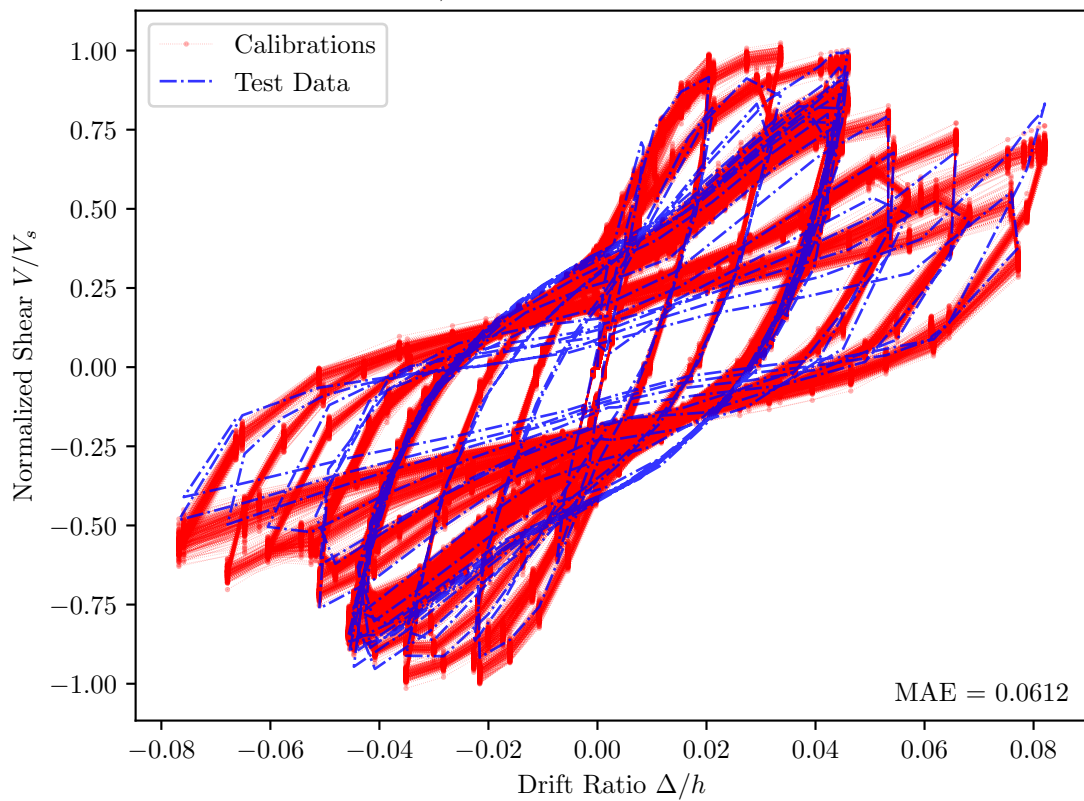
NIST, Model N6 — PEER Id = 313
