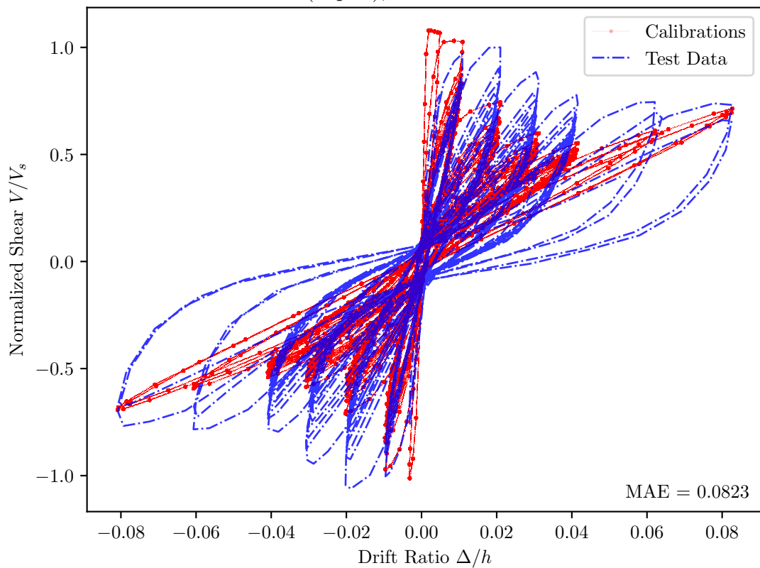
BRI No. 3 (Japan), ws21bs — PEER Id = 315
