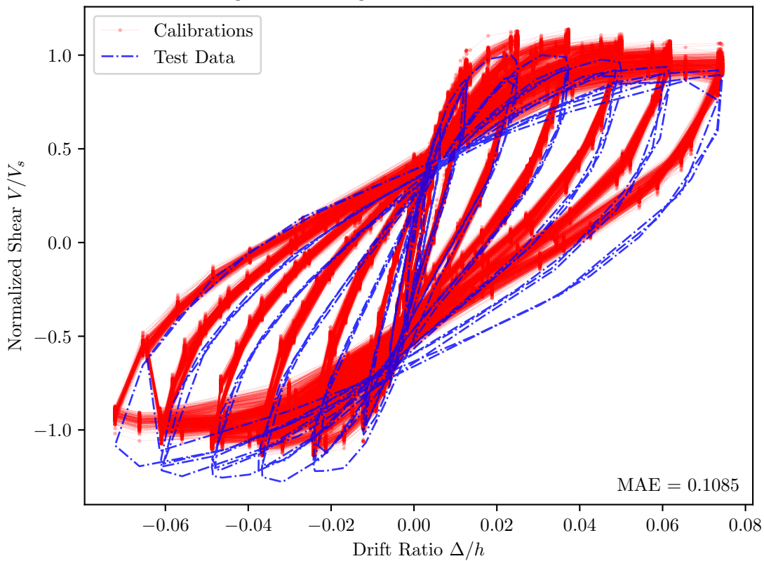
Saatcioglu and Baingo 1999, RC2 — PEER Id = 381
