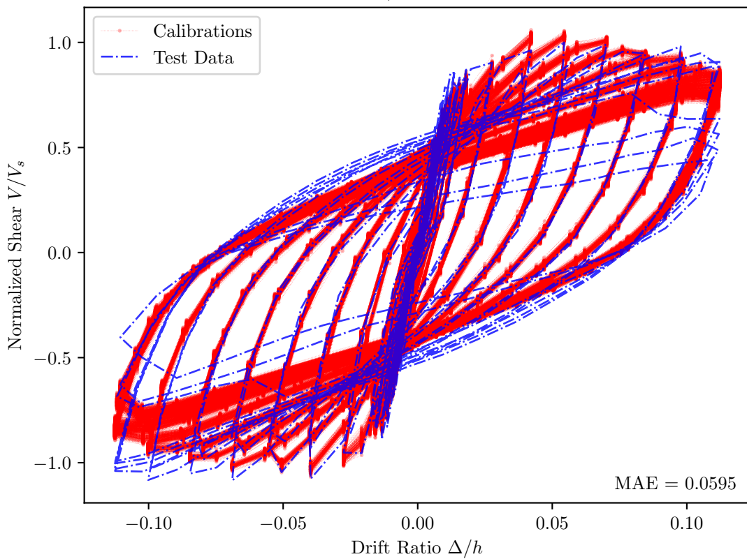
Soderstrom 2001,C2 — PEER Id = 396
