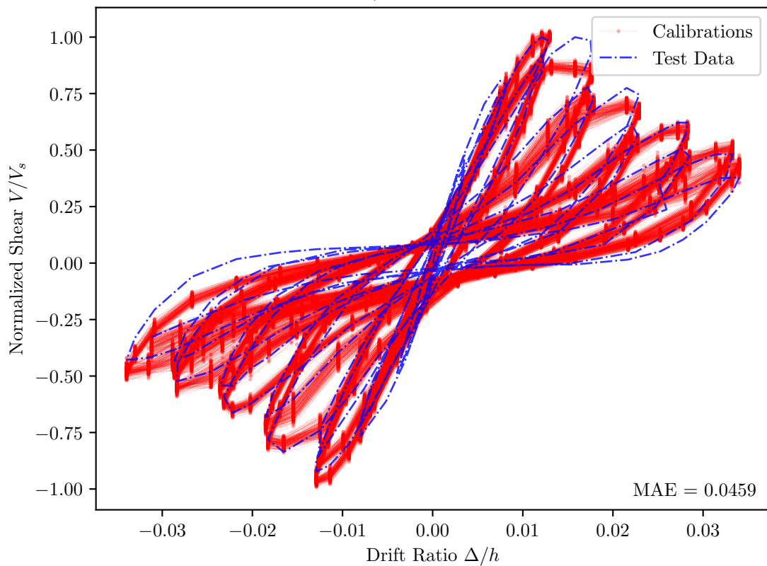
Ohue et al. 1985, 4D13RS — PEER Id = 034
