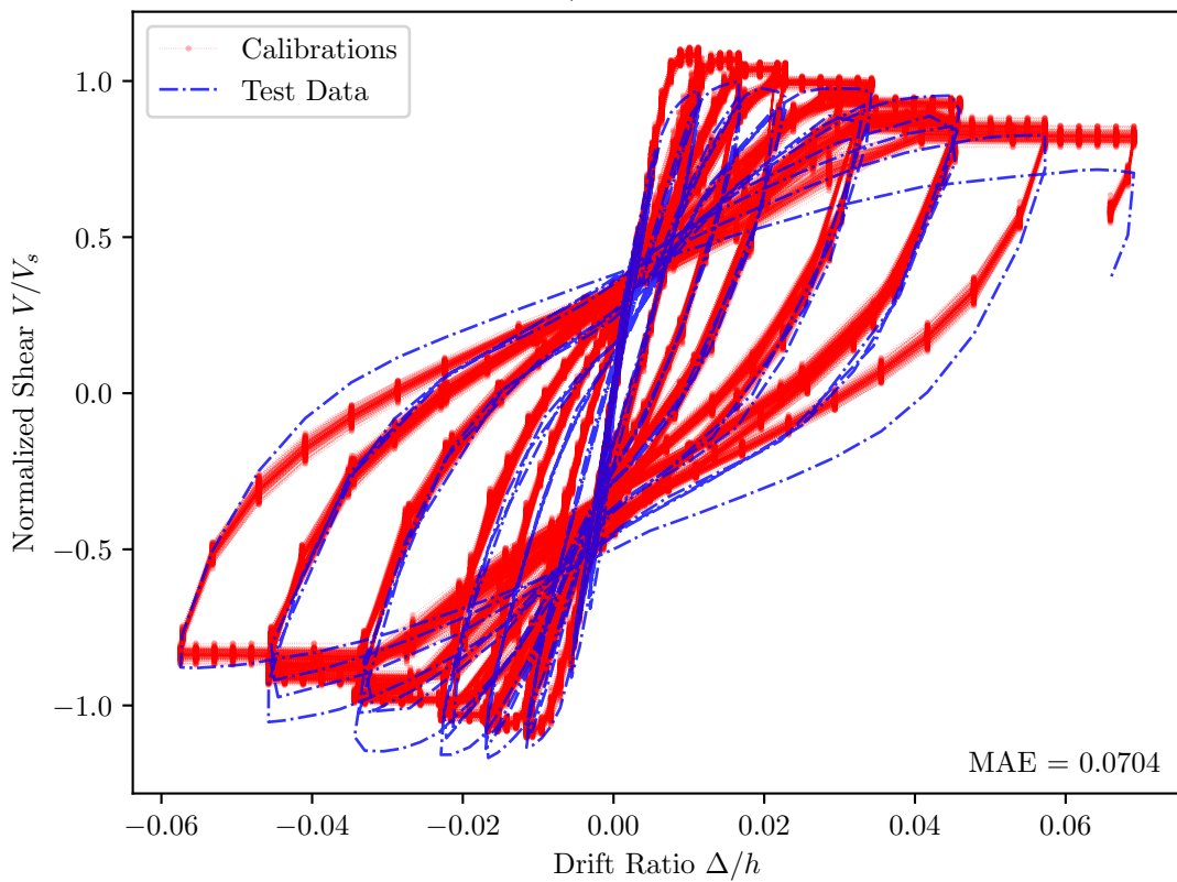
Kanda et al. 1988, 85STC-3 — PEER Id = 050
