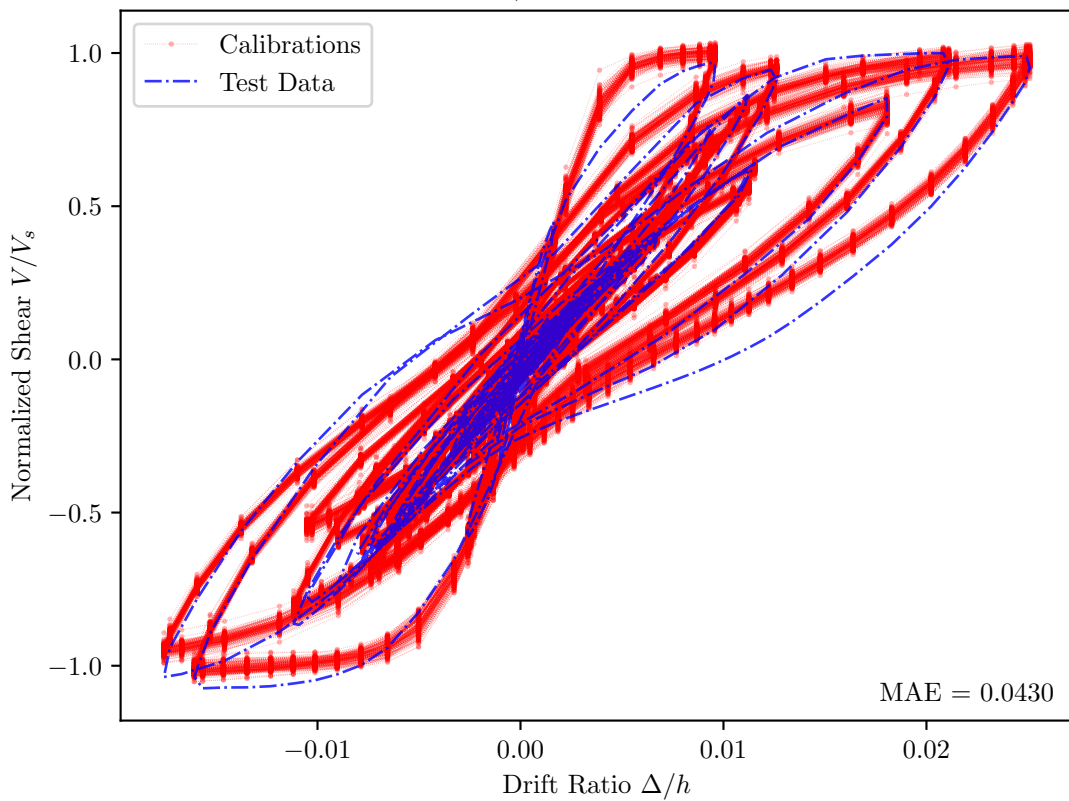
Kanda et al. 1988, 85PDC-2 — PEER Id = 052
