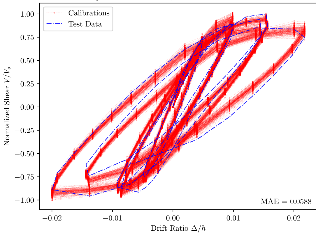
Muguruma et al. 1989, AL-2 — PEER Id = 058
