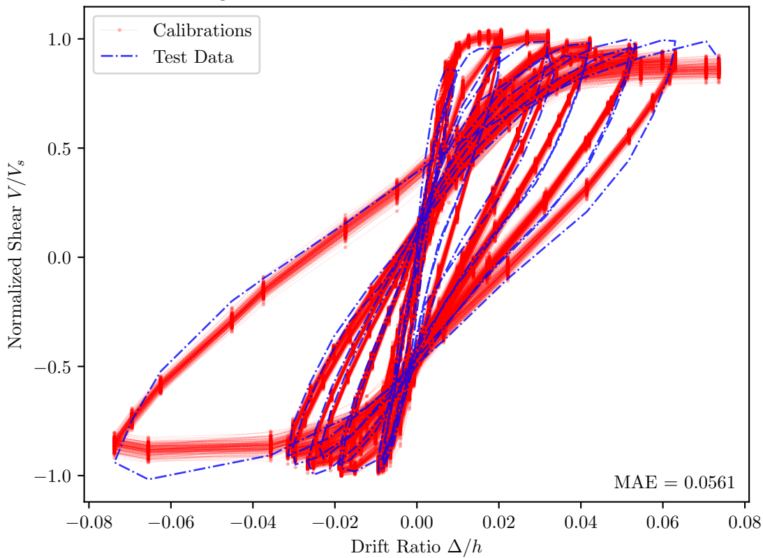
Muguruma et al. 1989, BL-1 — PEER Id = 060
