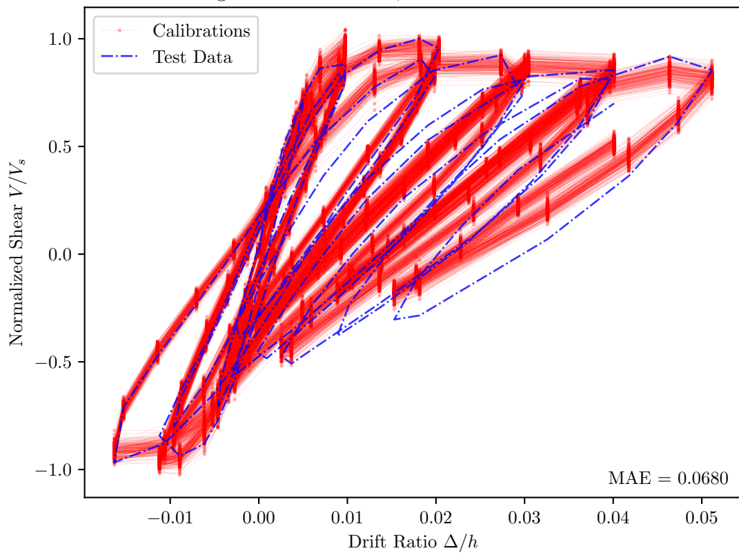
Muguruma et al. 1989, BL-2 — PEER Id = 062
