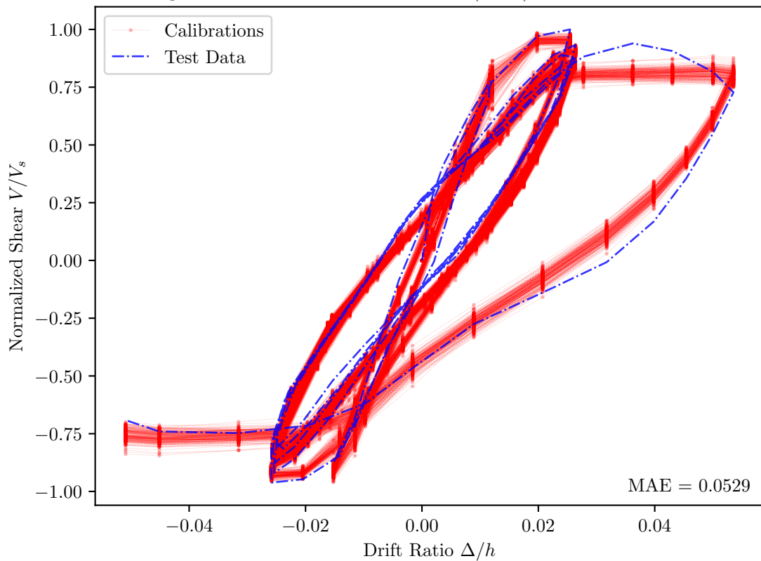
Wight and Sozen 1973, No. 40.033(East) — PEER Id = 078
