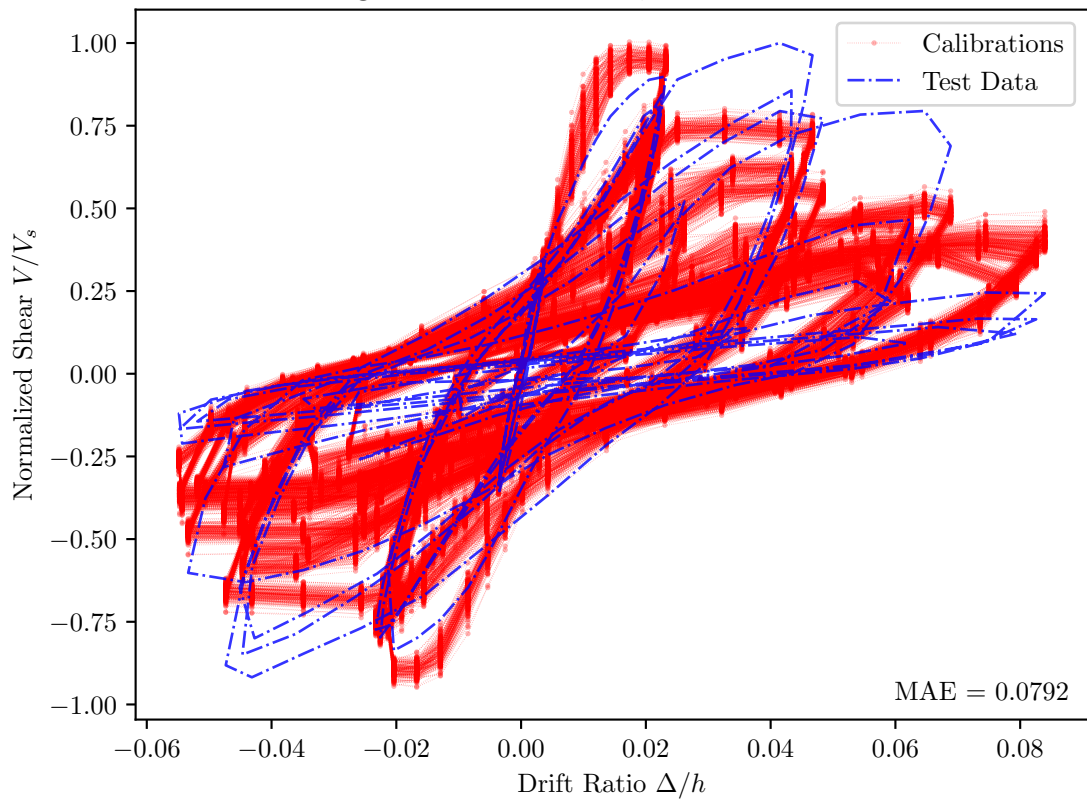
Saatcioglu and Ozcebe 1989, U1 — PEER Id = 104
