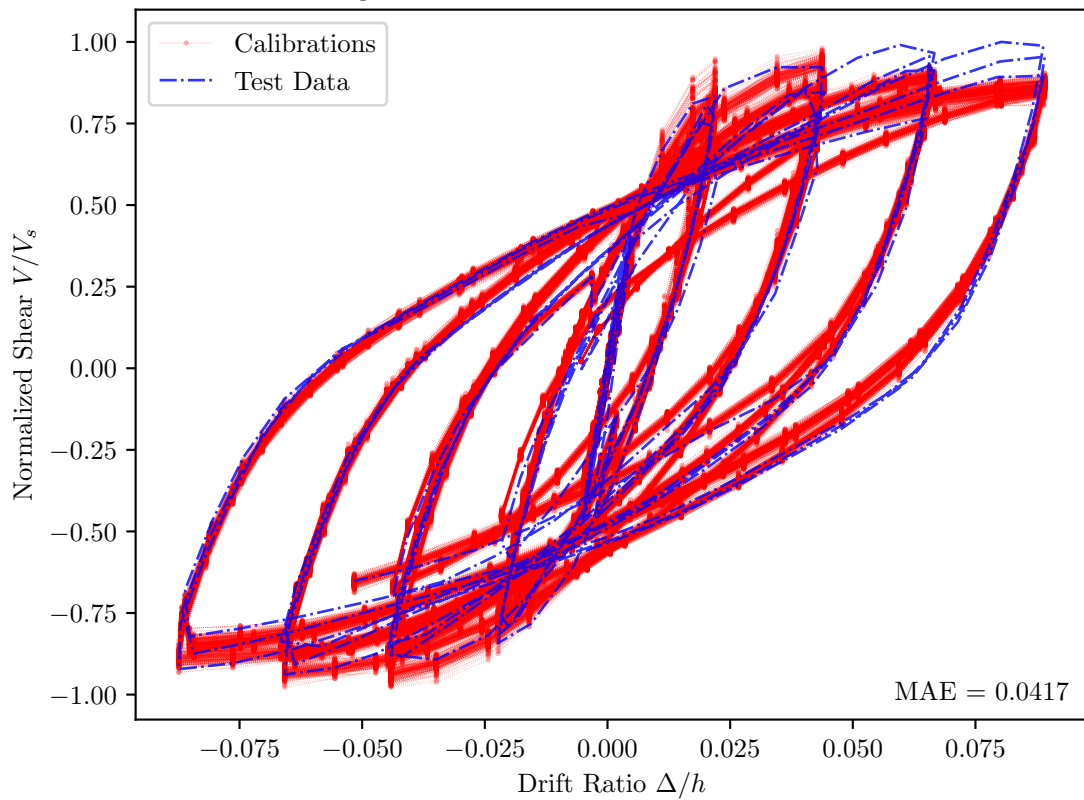
Saatcioglu and Ozcebe 1989, U6 — PEER Id = 107
