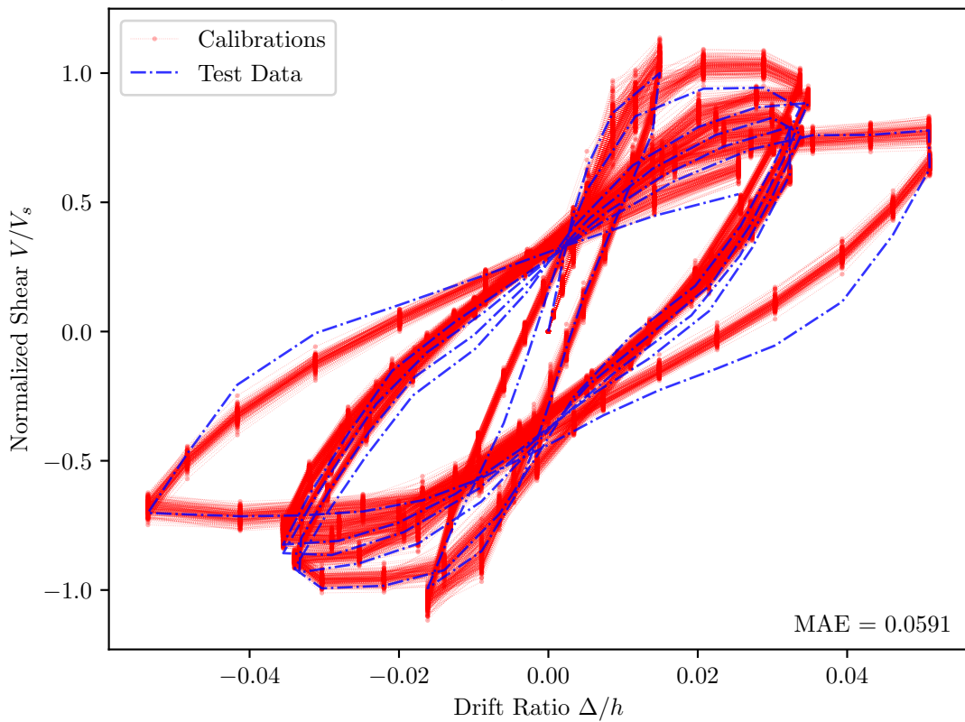
Galeota et al. 1996, CA4 — PEER Id = 120
