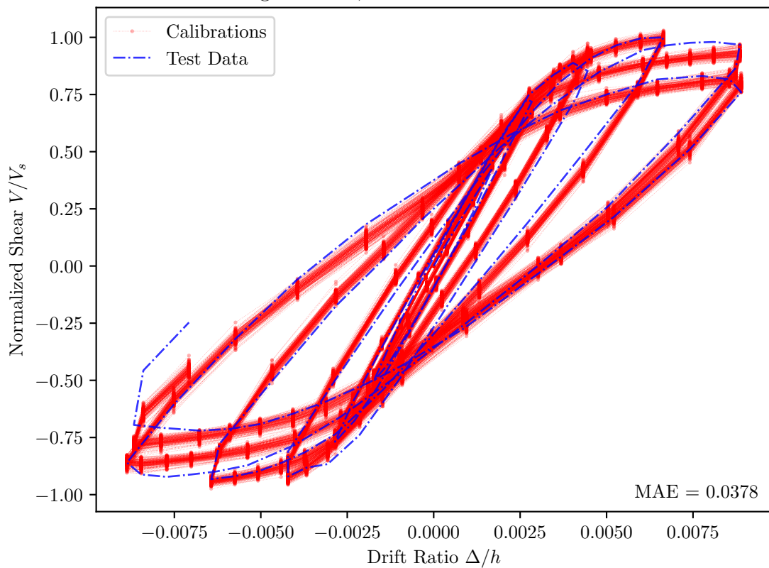
Sugano 1996, UC10H — PEER Id = 151
